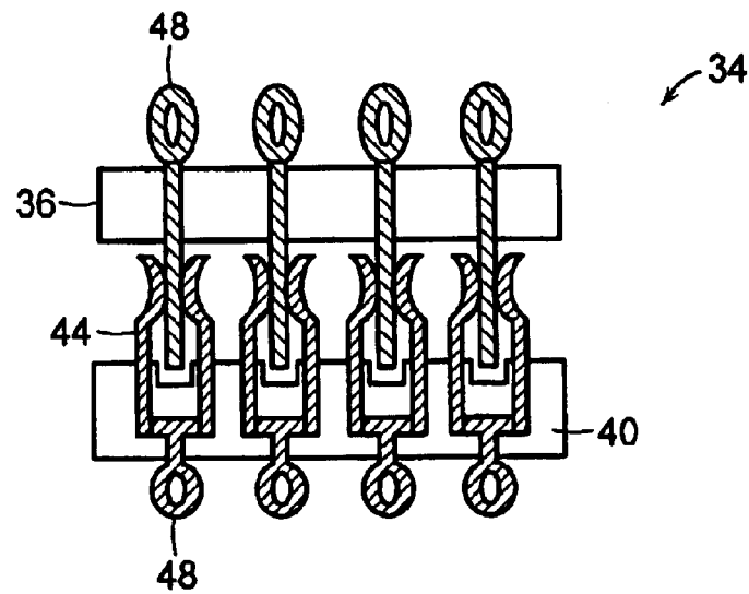
FIG. 3A (RELATED ART)
