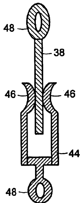
FIG. 3B (RELATED ART)
