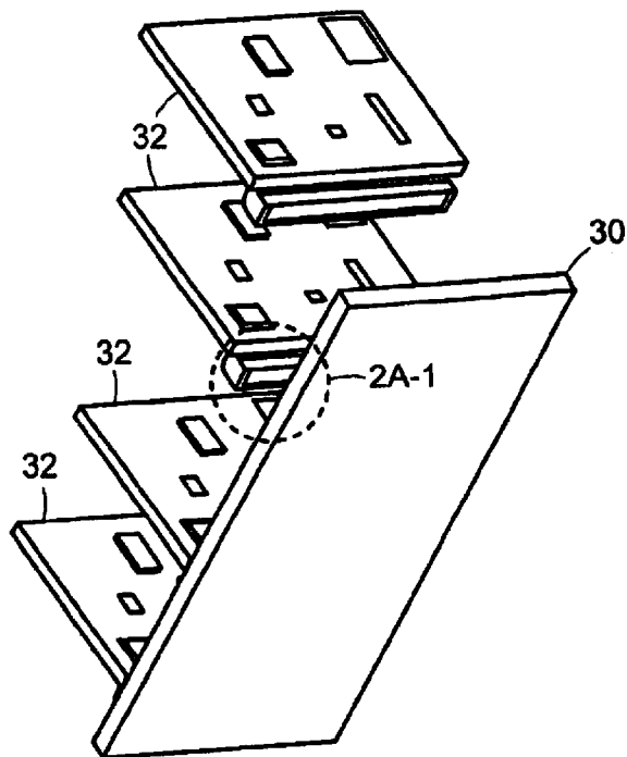
FIG. 2A (RELATED ART)
