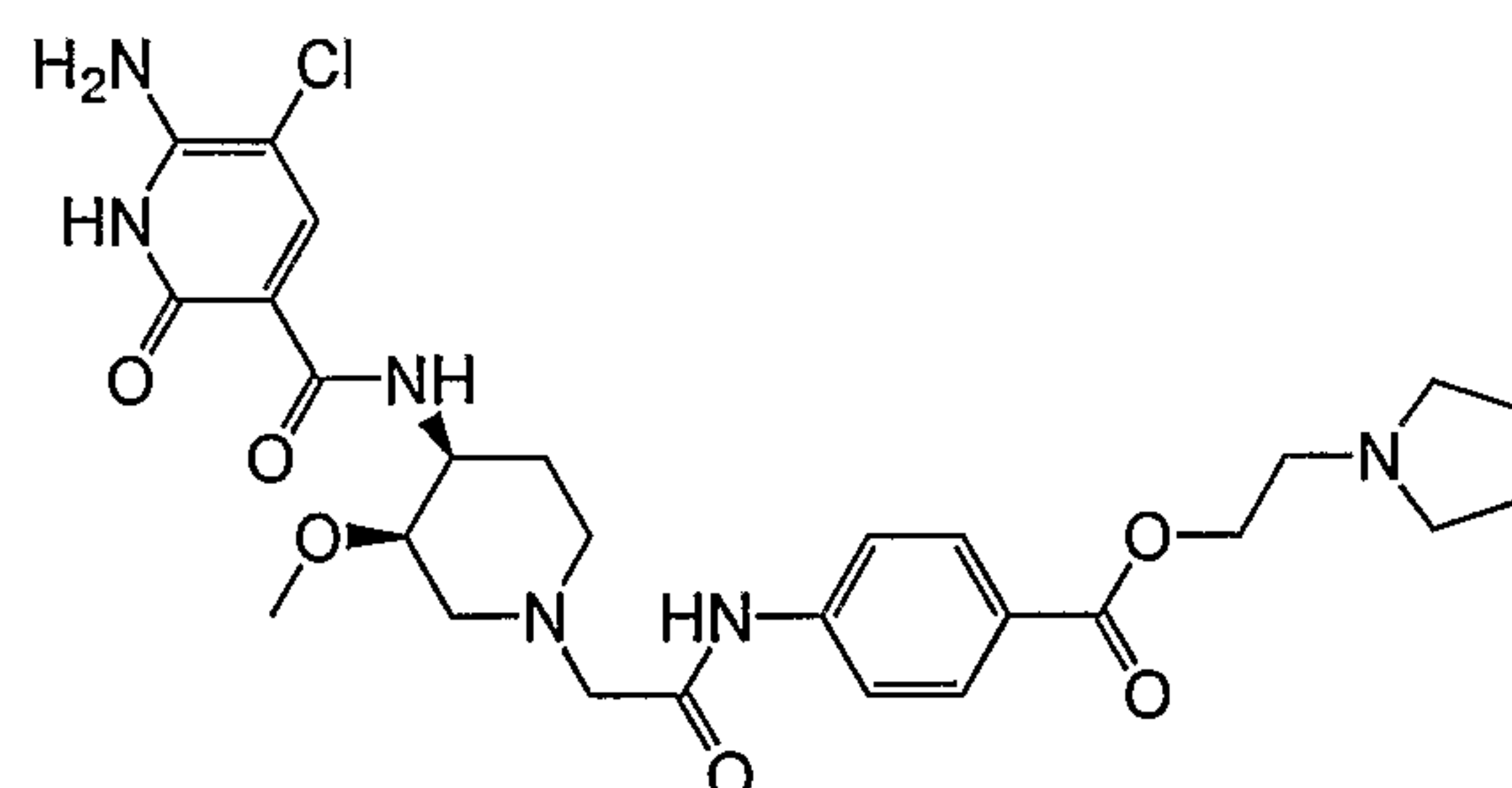
2-(pyrrolidin-1-yl)ethyl 4-(2-((3 R ,4 S )-4-(6-amino-5-chloro-2-oxo-1,2-dihydropyridine-3-carboxamido)-3-methoxypiperidin-1-yl)acetamido)benzoate
