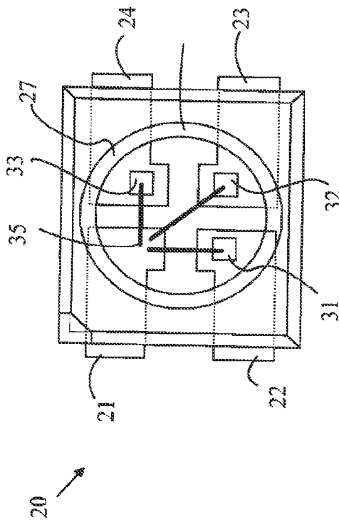
FIGURE 3 (PRIOR ART)
