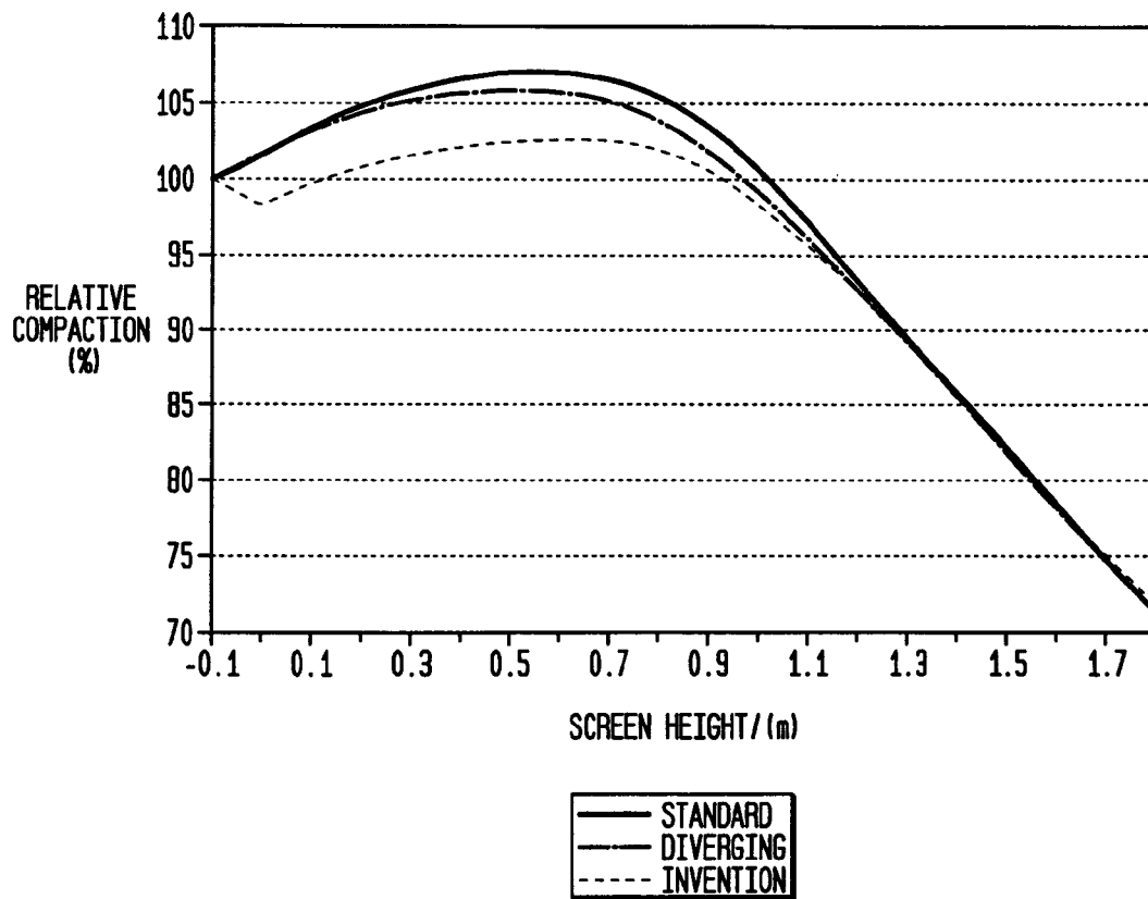
FIG. 12 RELATIVE CHIP COLUMN COMPACTION
