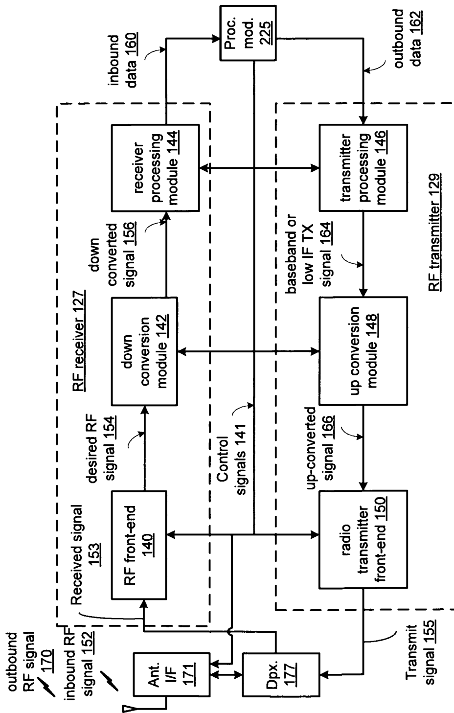
RF transceiver 123
