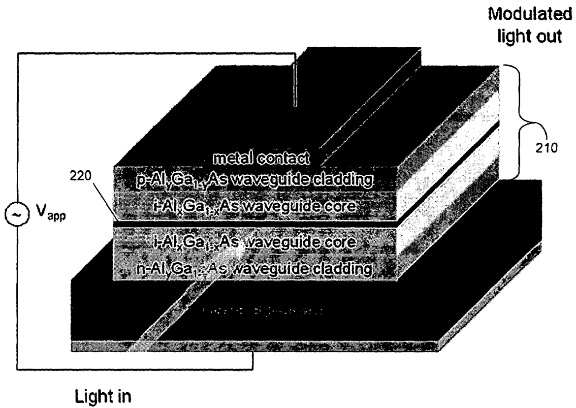
FIG. 2 (PRIOR ART)
