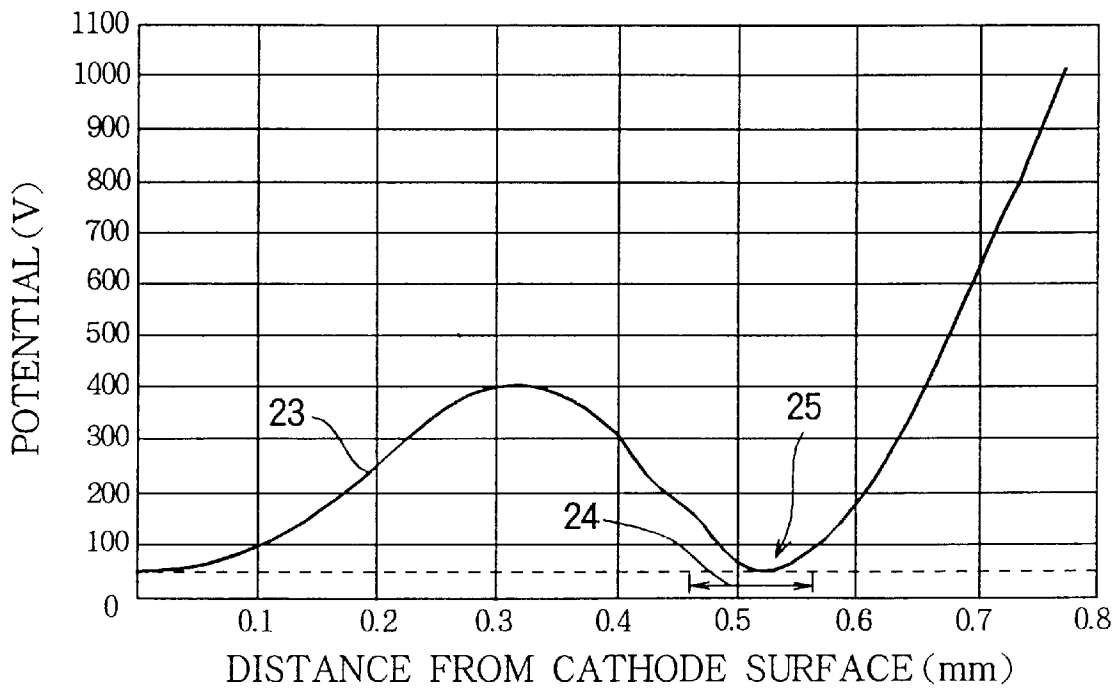
FIG. 6 PRIOR ART
