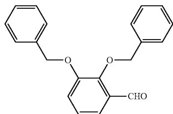
2,3-bis(benzyloxy)benzaldehyde
