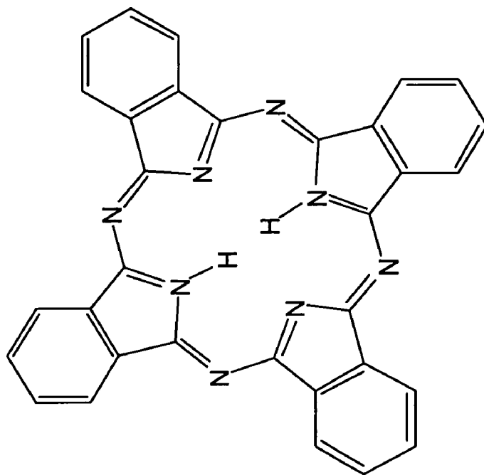
Metal-free Phthalocyanine
