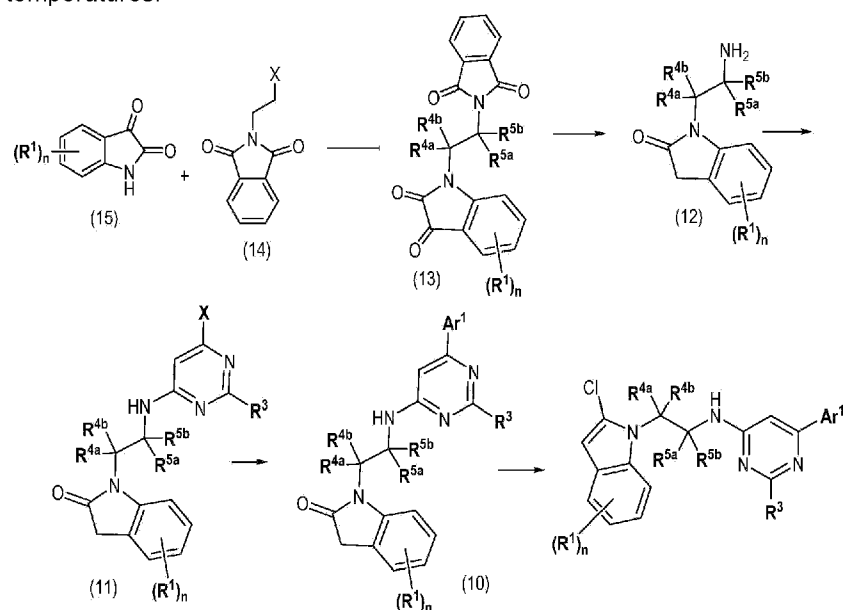
Scheme 7
