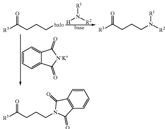
Synthetic Scheme III
