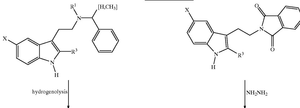
Synthetic Scheme IV
