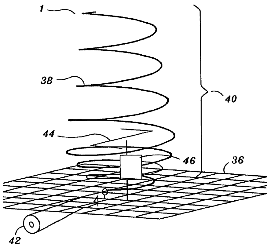
HELIX WITH Z-SHAPED DIPOLE
