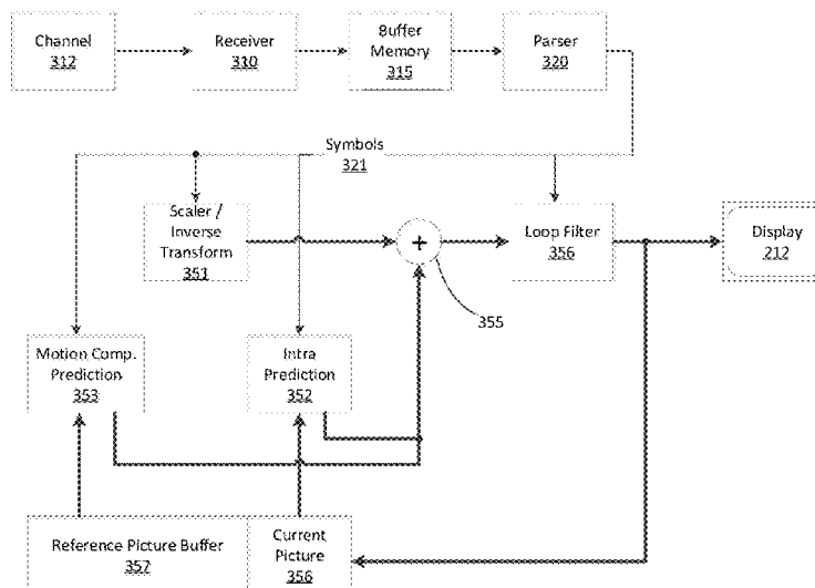
Decoder 210
