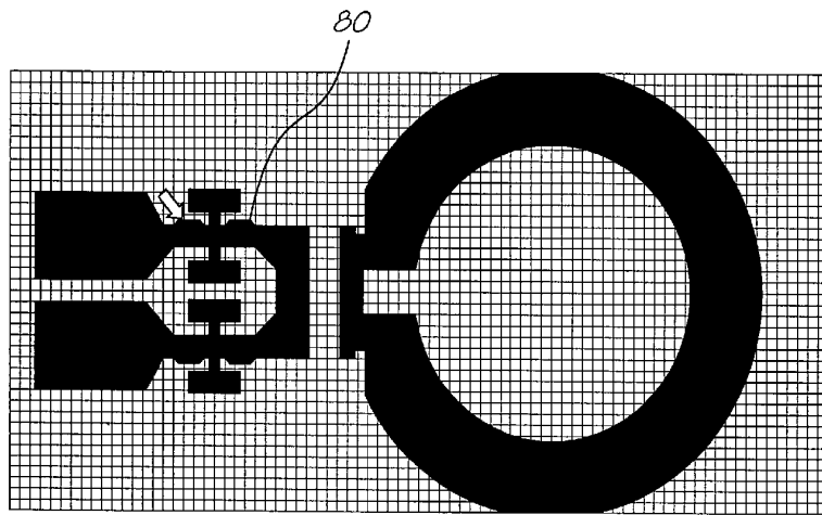
Top view of actuator layer (mask 4)
