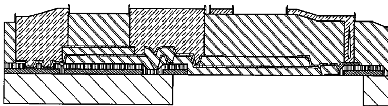
Side view including sacrificial layers
