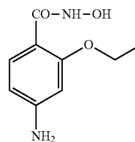
2-ethoxy-4-amino benzoylhydroxamic acid
