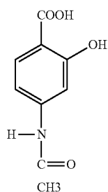
4-acetylamino salicylic acid
