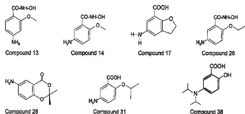
Structures of Compounds 13, 14, 17, 26, 31 and 38
