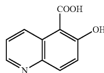
6-hydroxy-quinoline-5-carboxylic acid
