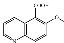
6-methoxy quinoline-5-carboxylic acid
