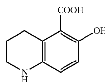
1,2,3,4-tetrahydro-6-hydroxy quinoline-5-carboxylic acid
