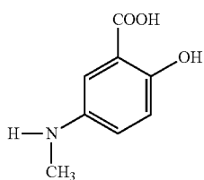
5-methylamino salicylic acid
