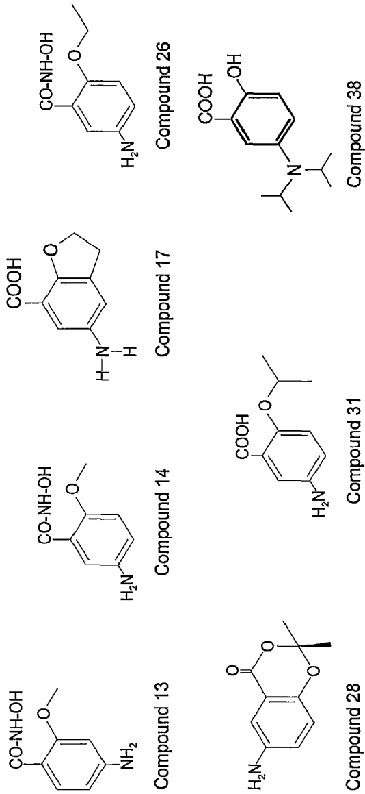
Fig. 1A: Structures of Compounds 13, 14, 17, 26, 31 and 38
