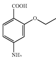
2-ethoxy-4-aminobenzoic acid
