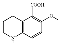
6-methoxy-1,2,3,4-tetrahydro quinoline-5-carboxylic acid
