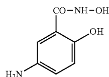
5-amino salicylhydroxamic acid
