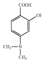
4-dimethylamino salicylic acid
