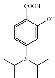
4-diisopropylamino salicylic acid
