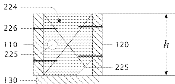
FIG. 2b end view
