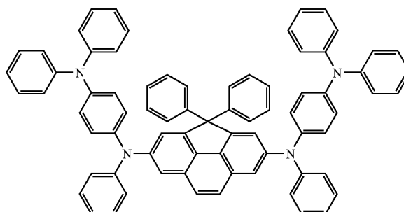
<Formula 35>
