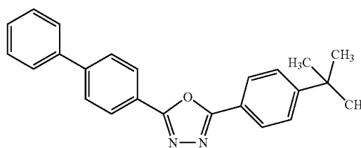
Oxadiazole-containing compound
