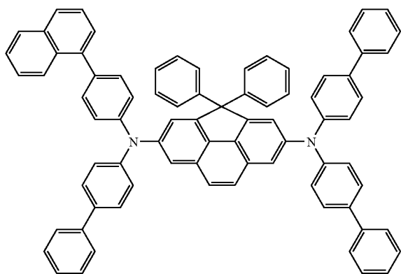
<Formula 30>
