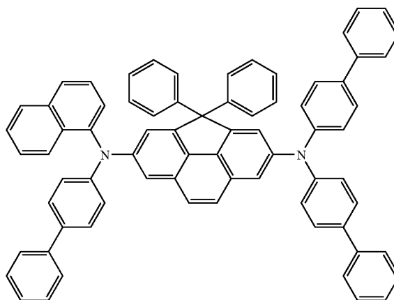
<Formula 29>
