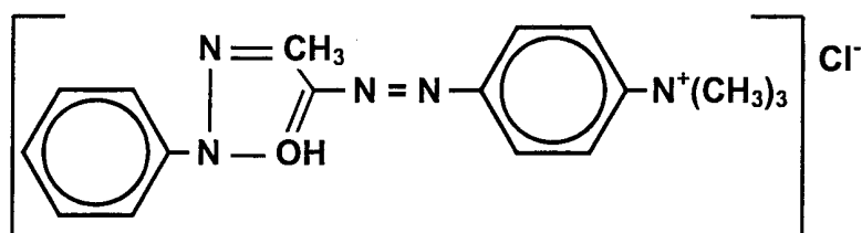
Formula 4: Basic Yellow 57
