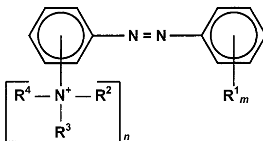
Formula 1: Basic Azo Dyes
