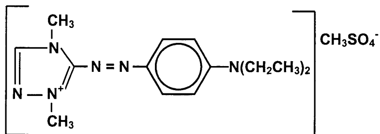
Formula 3: Basic Red 46
