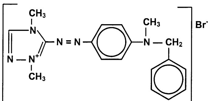
Formula 3: Basic Red 46
