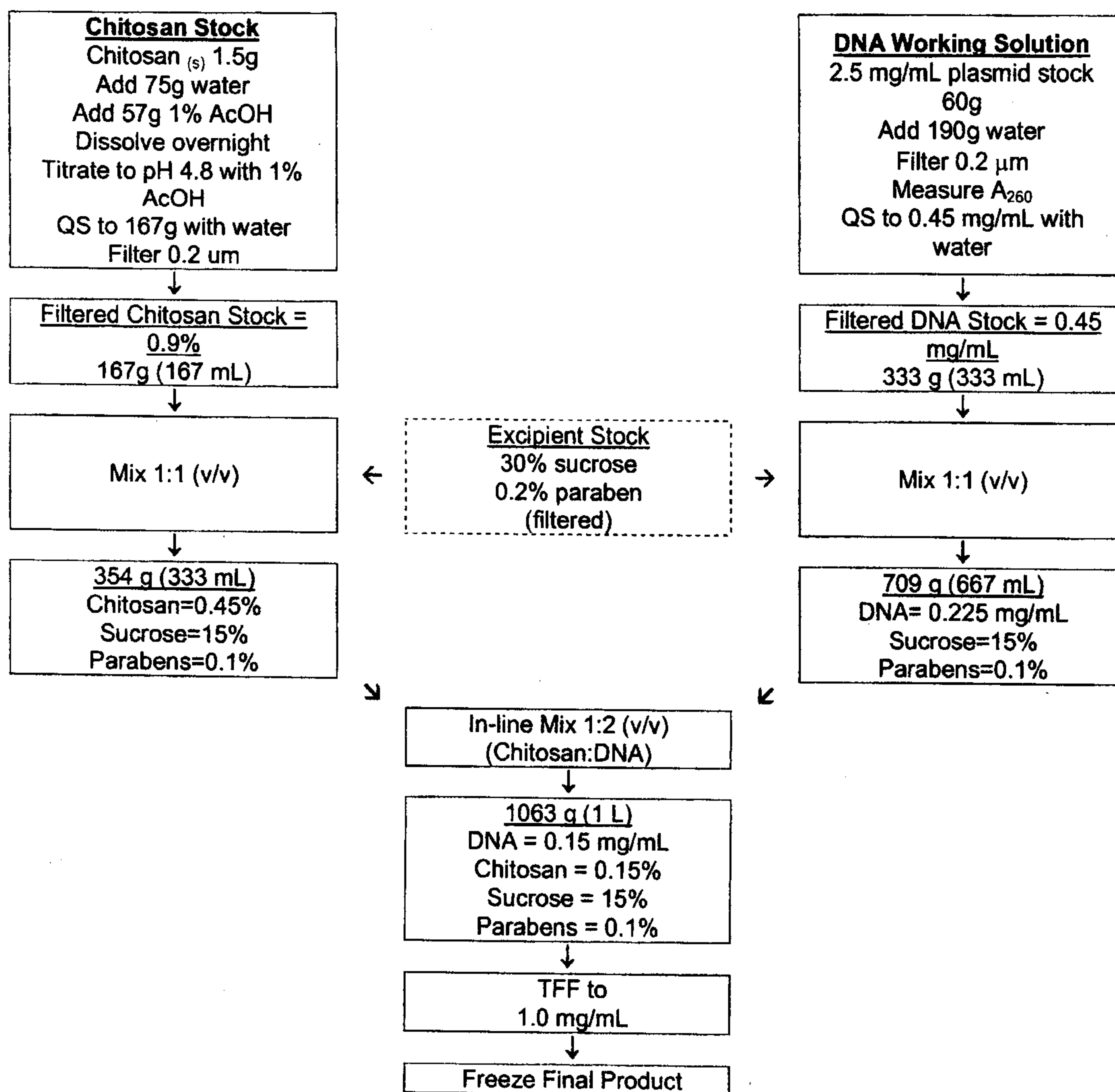
Figure 1: Process Block for 1L In-line Mixing Batch and Concentration
