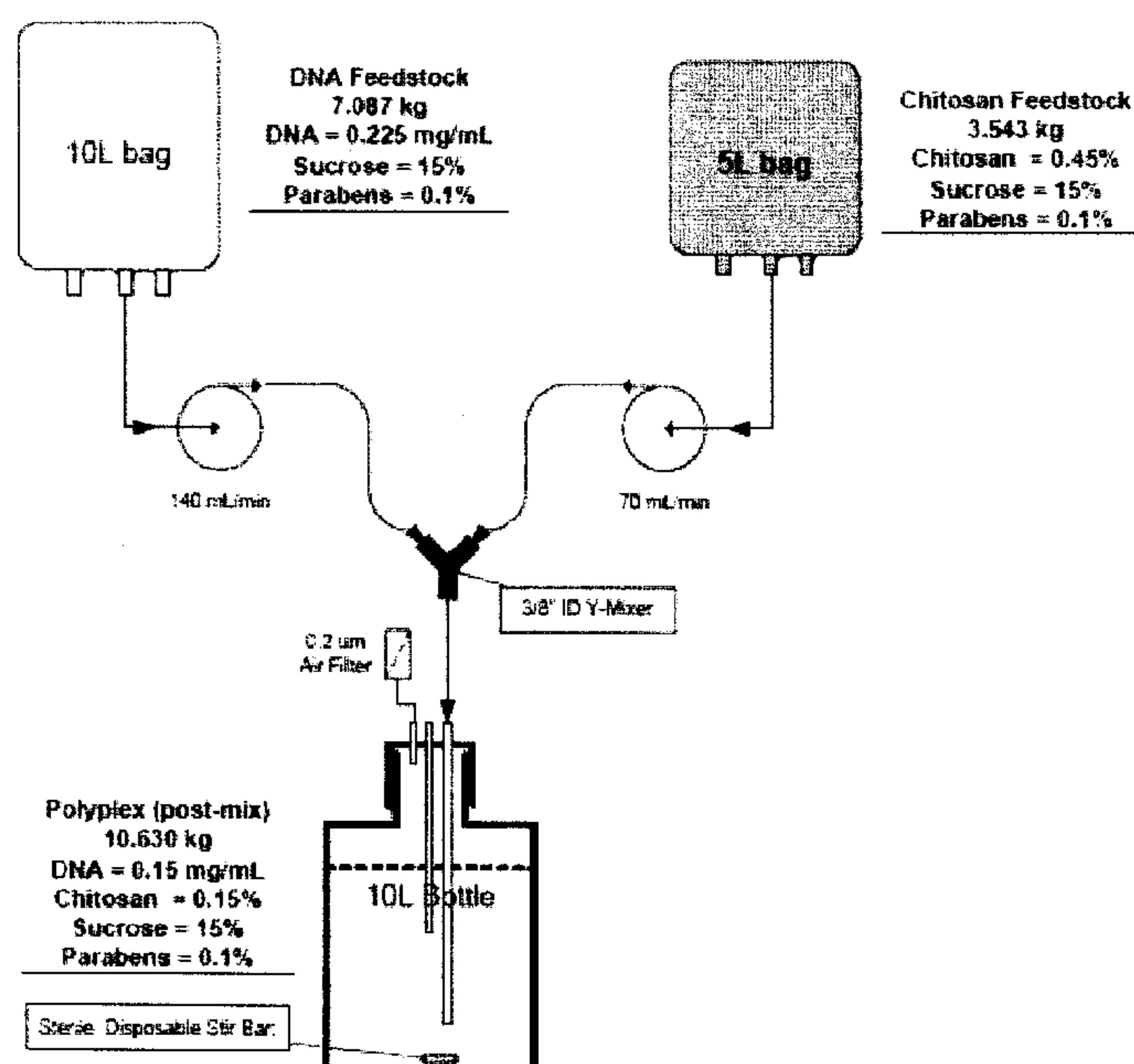
Figure 3: Mid-Scale In-line Mixing Schematic for 10L
