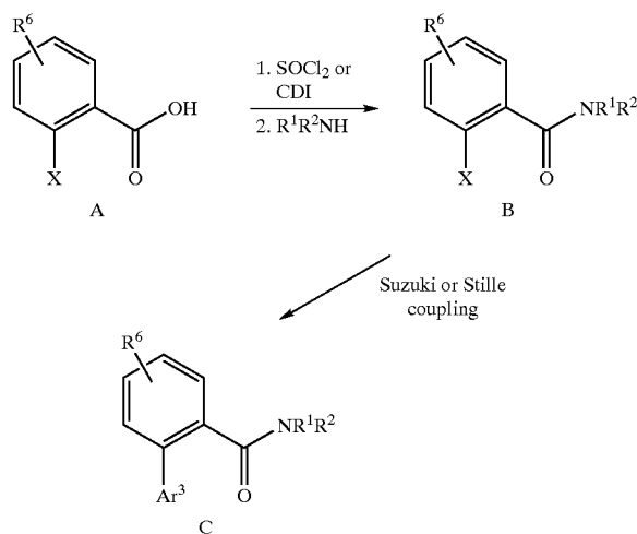
Scheme 1. Preparation of Ortho Biarylamides
