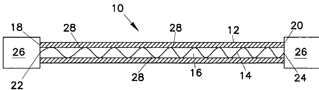
FIG. 3 (PRIOR ART)
