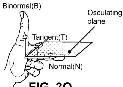
Left-hand rule
