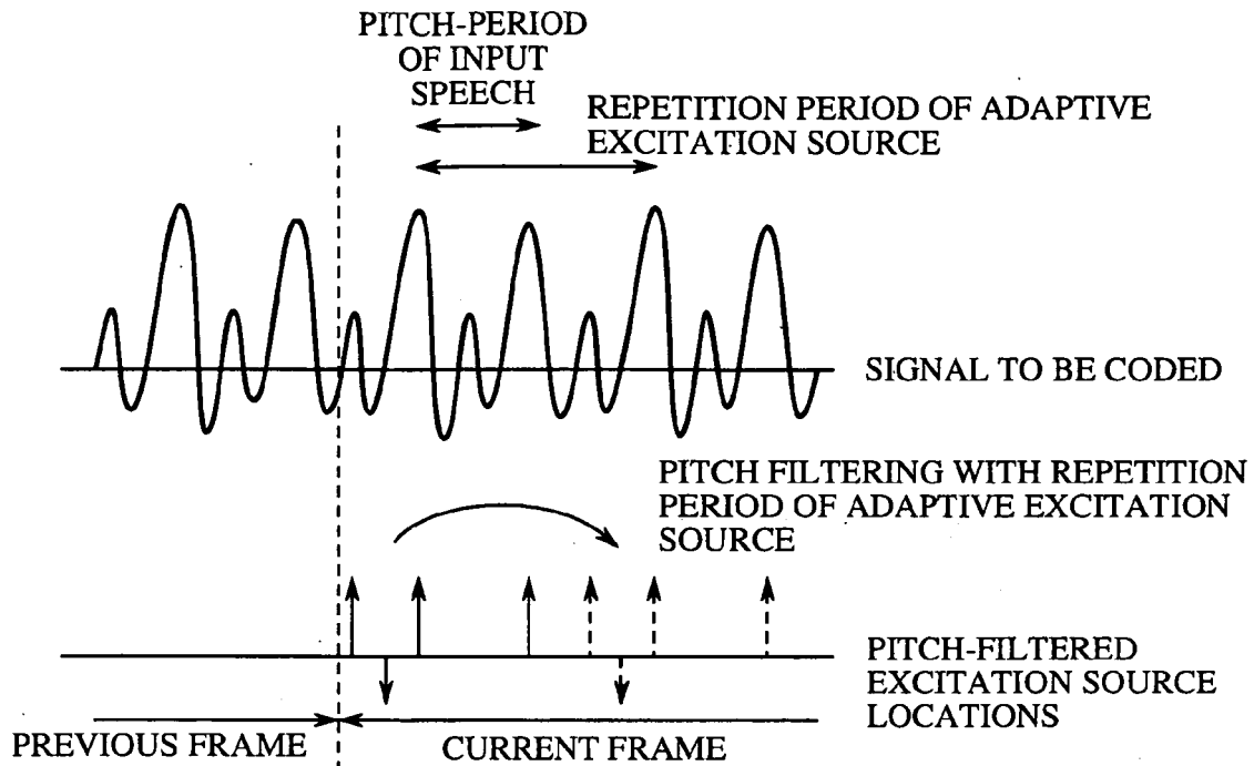
FIG.18 (PRIOR ART)
