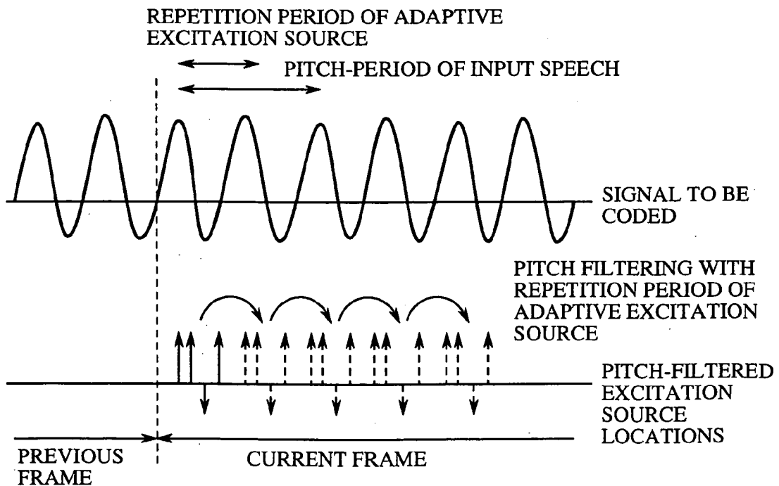
FIG.19 (PRIOR ART)
