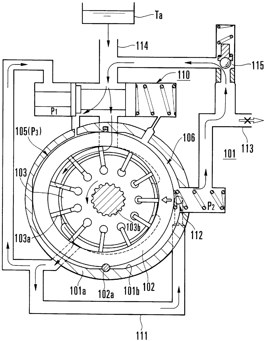
FIG. 27 PRIOR ART
