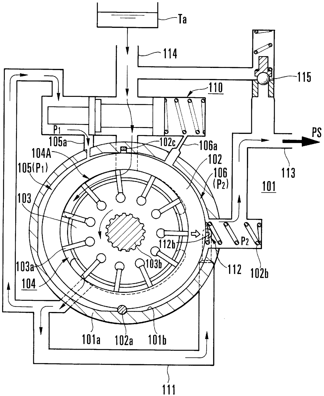
FIG. 26 PRIOR ART
