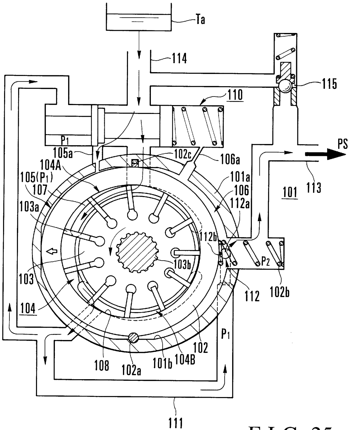
FIG. 25 PRIOR ART
