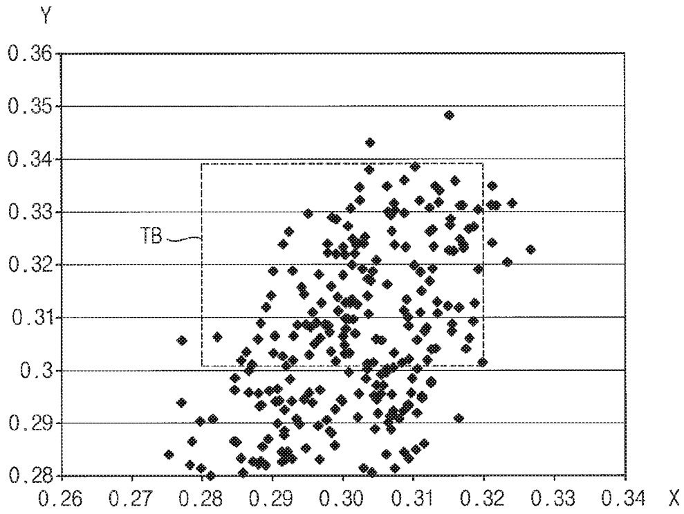
FIG. 9 (PRIOR ART)
