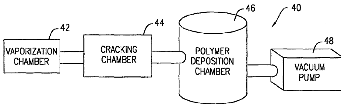
PARYLENE VACUUM EVAPORATION REACTOR
