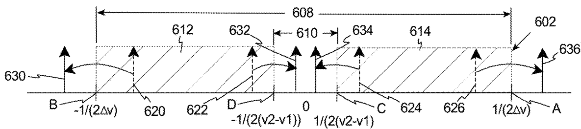
Fourier Space
