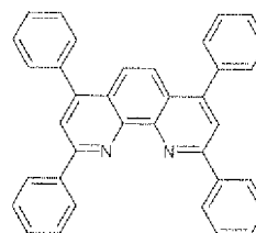
2,4,7,9-tetraphenyl-1,10-phenanthroline, CAS 51786-73-3, -2.33 V, G4;
