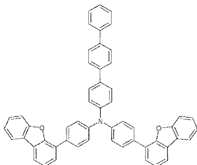
N,N-bis(4-(dibenzo[b,d]furan-4-yl)phenyl)-[1,1':4',1''-terphenyl]-4-amine (NHT-195), CAS 1198399-61-9, A2;
