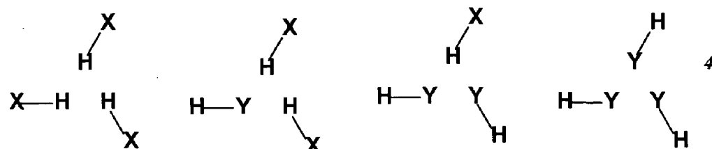
Tricarboxylic Acid Tricarboxylic Acid Tricarboxylic Acid Tricarboxylic Acid
