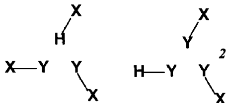
Pentacarboxylic Acid Pentacarboxylic Acid
