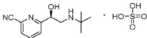
Compound 3
