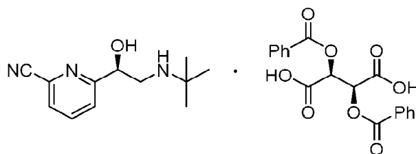
Compound 14
