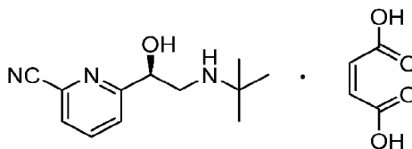
Compound 6
