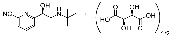
Compound 9 Form A
