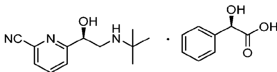
Compound 11
