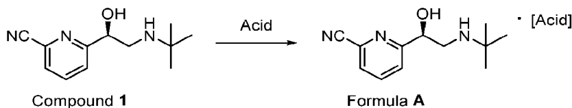
Scheme 2. Preparation of Salts of Formula A
