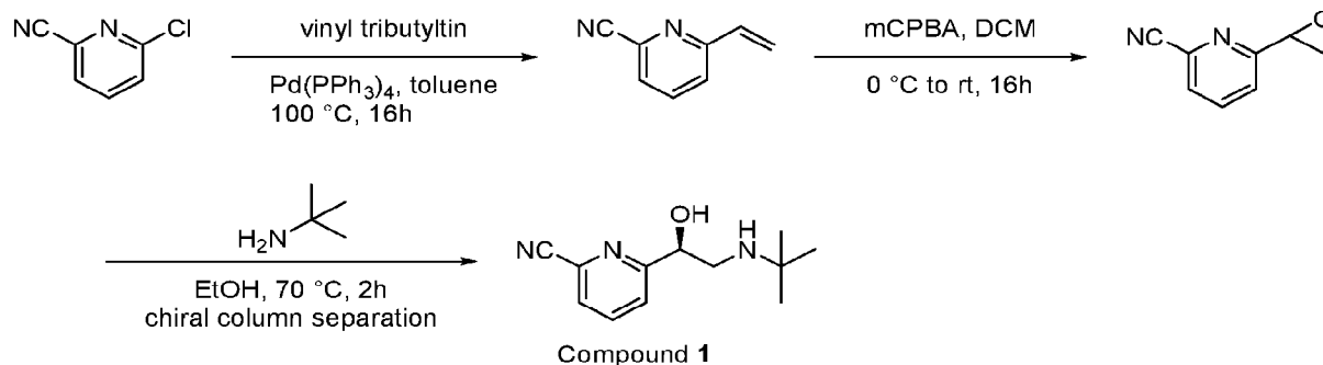
Scheme 1. Preparation of Compound 1
