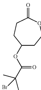
7-Oxo-oxepan-4-yl 2-bromo-2- methylpropanoate (BMP-XO)
