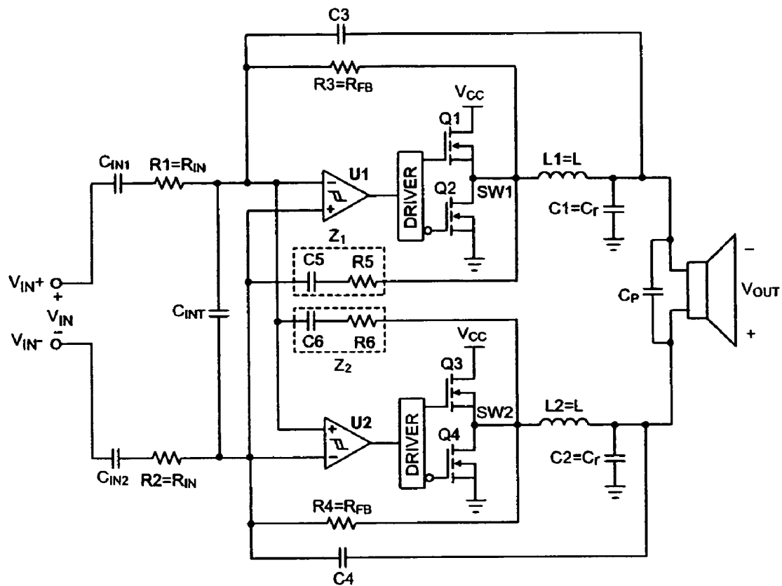
Figure 3 - BTL Audio Amplifier using Two Comparators
