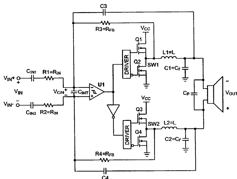
BTL Audio Amplifier with Single Comparator
