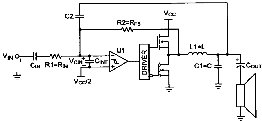
Figure 1 - Single Ended Class D Audio Amplifier (Prior Art)
