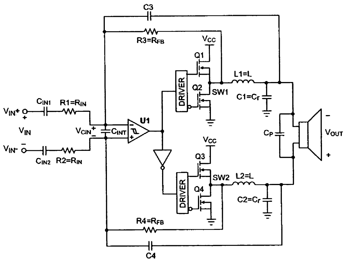
Figure 2 - BTL Audio Amplifier with Single Comparator
