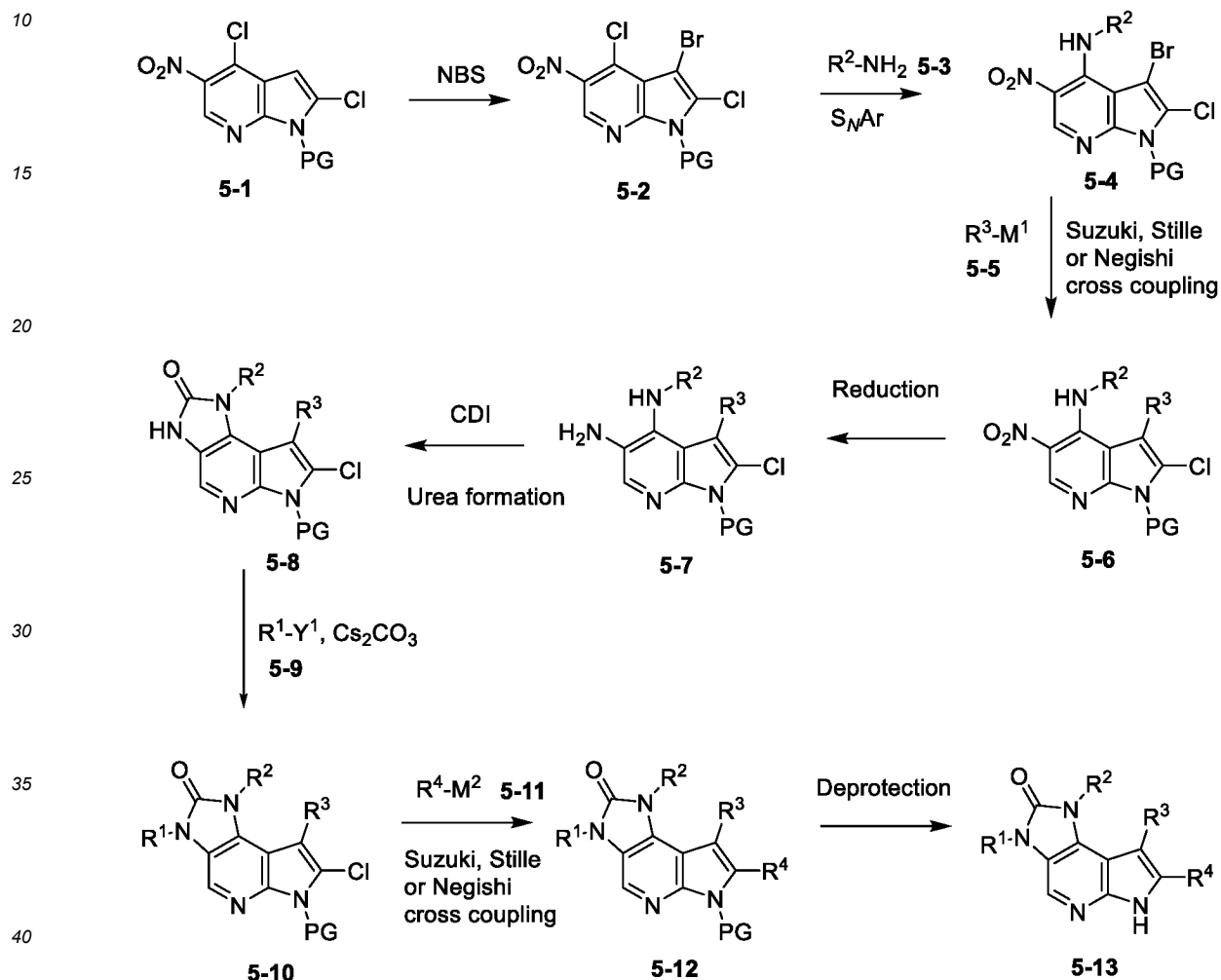
Scheme 5.
