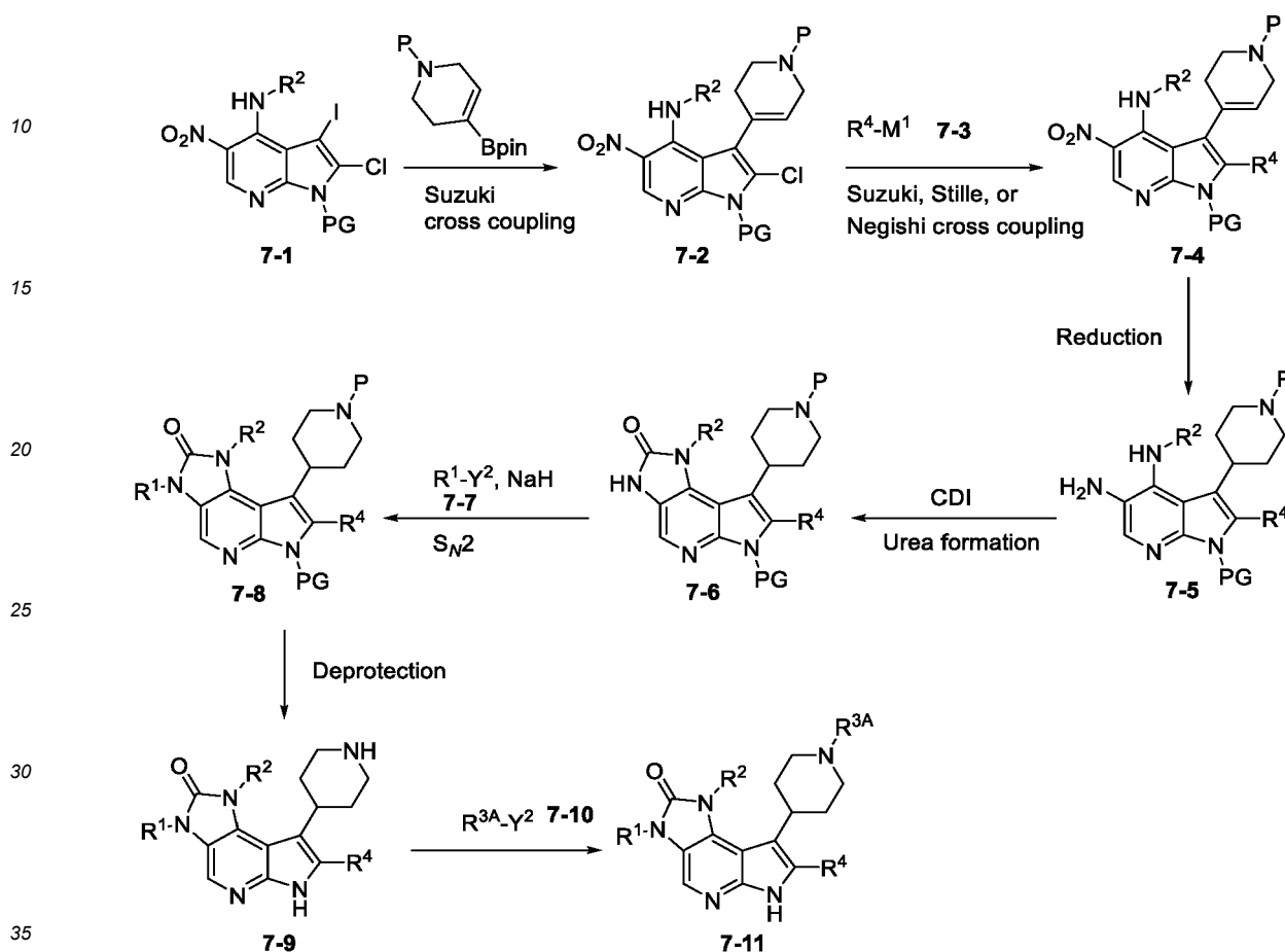
Scheme 7.
