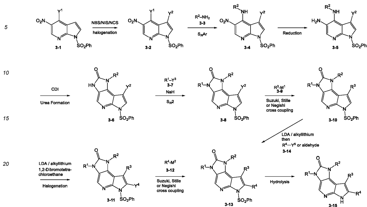
Scheme 3.
