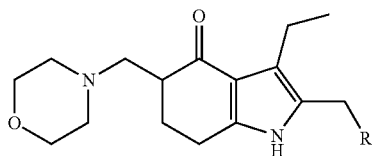
R''' = —OH, alkoxy, alkyl, substituted alkyl
