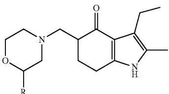
R = —OH, alkoxy, alkyl, substituted alkyl
