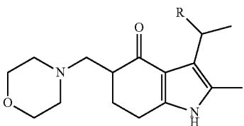
R = —OH, alkoxy, alkyl, substituted alkyl
