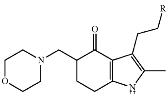
R = —OH, alkoxy, alkyl, substituted alkyl
