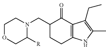
R = —OH, alkoxy, alkyl, substituted alkyl
