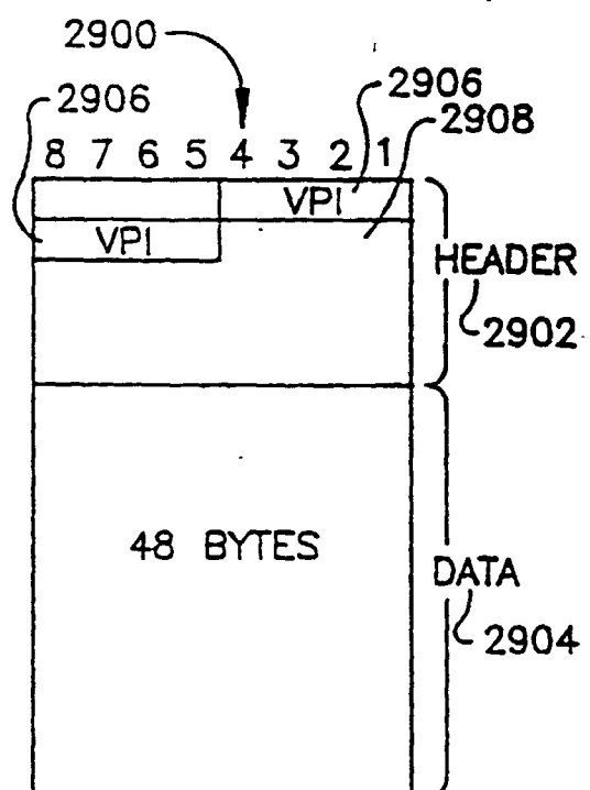
TDM CELL Fig. 29
