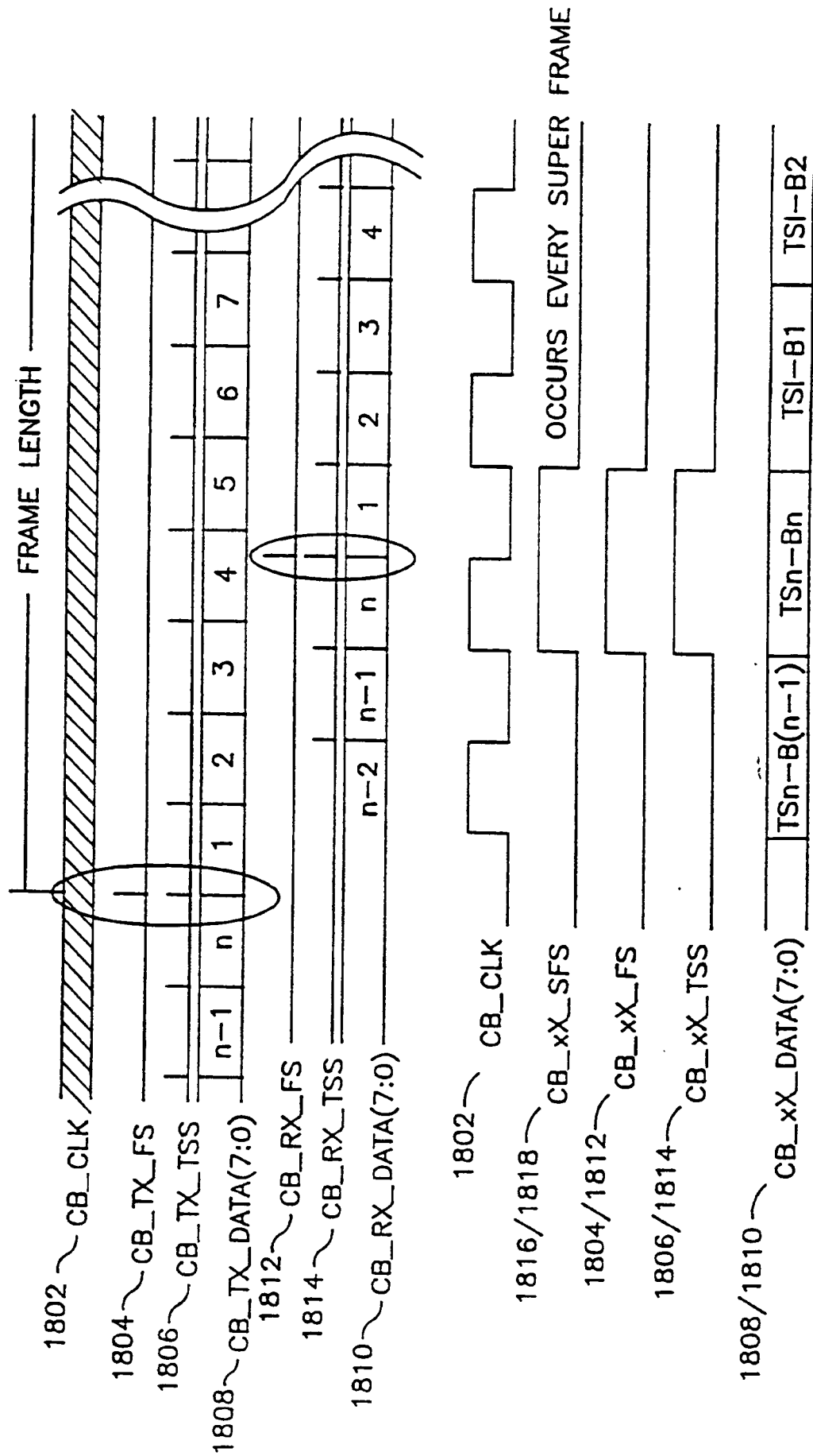
Fig. 18 CELL BUS TIMING
