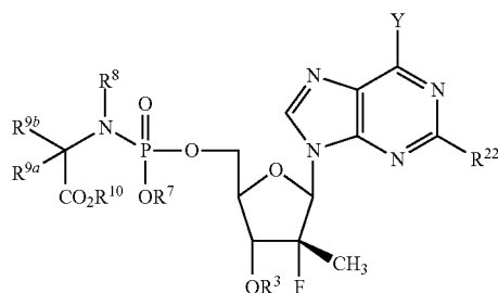
Formula IV
