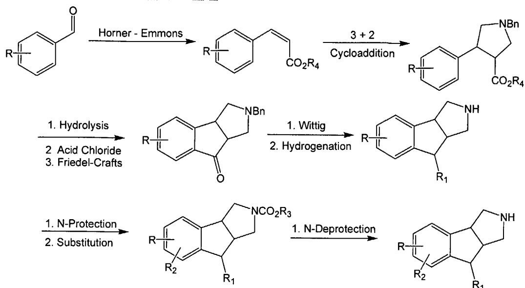
Scheme 3. Synthesis of 8-Substituted-Indeno-pyrroles via a 3+2 cycloaddition on substituted cis -substituted-phenyl acrylic acid ethyl esters.
