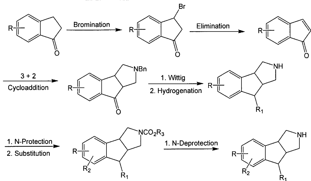
Scheme 1. Synthesis of 8-Substituted-Indeno-pyrroles via a 3+2 cycloaddition on substituted indenones.
