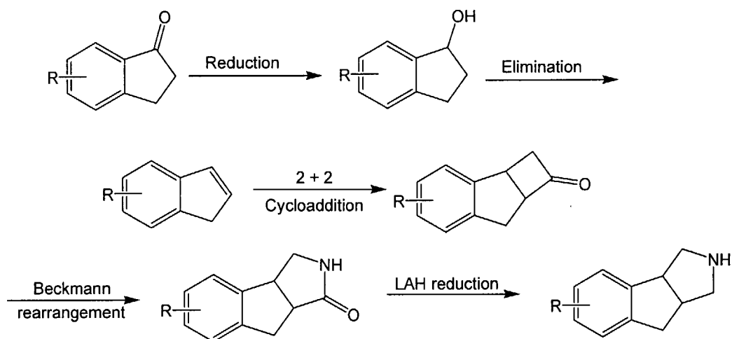
Scheme 2. Synthesis of Indeno-pyrroles via a Beckmann rearrangement on substituted indenenes.
