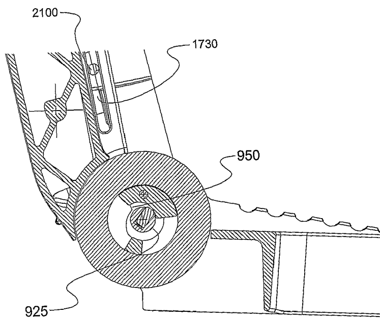
SECTION G - G
