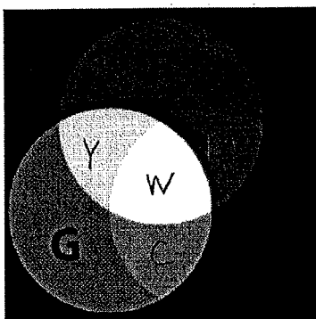
Additive color mixing: adding red to green yields yellow; adding all three primary colors together yields white.
