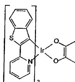
Btp 2 (acac)
