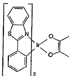
Bt 2 (acac)
