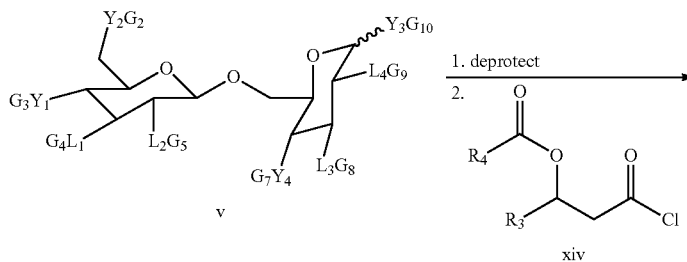
Reaction Scheme 3
