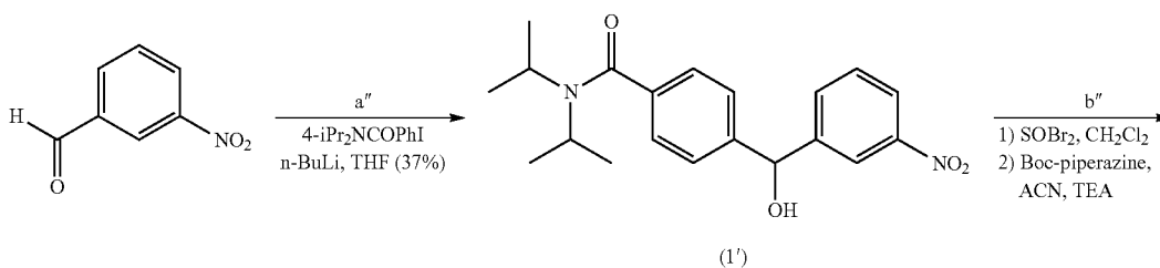
Scheme 3: Preparation of Methyl Sulfonilides; Examples 7-8
