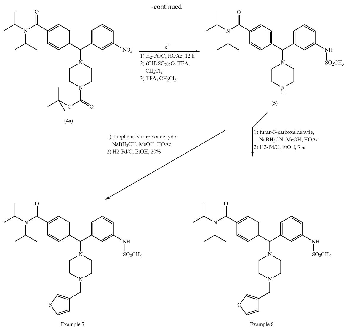
Intermediate 5: N,N-diisopropyl-4-[(3-[(methylsulfonyl)amino]phenyl)(1-piperazinyl)methyl]benzamide
