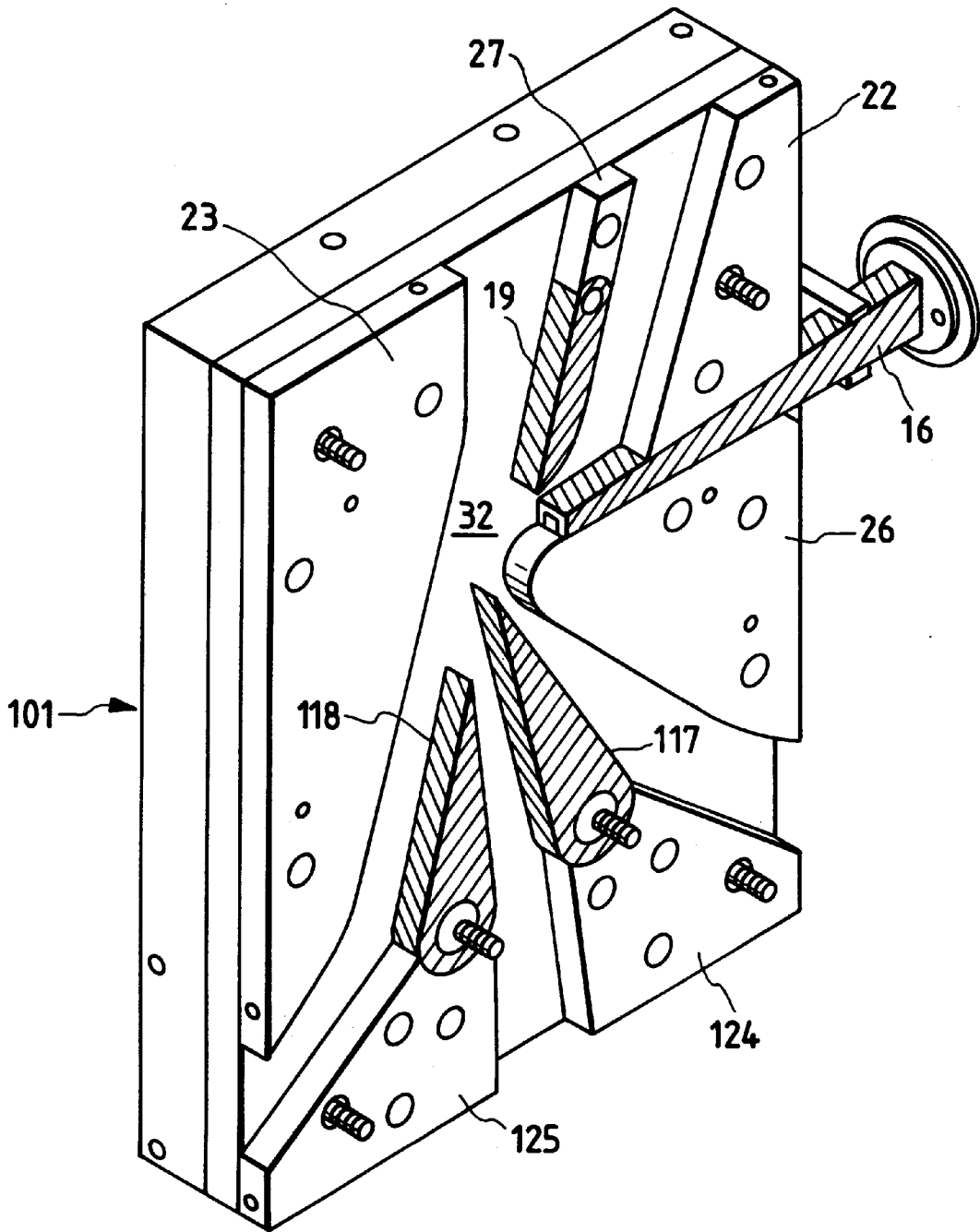
FIG. 16 PRIOR ART
