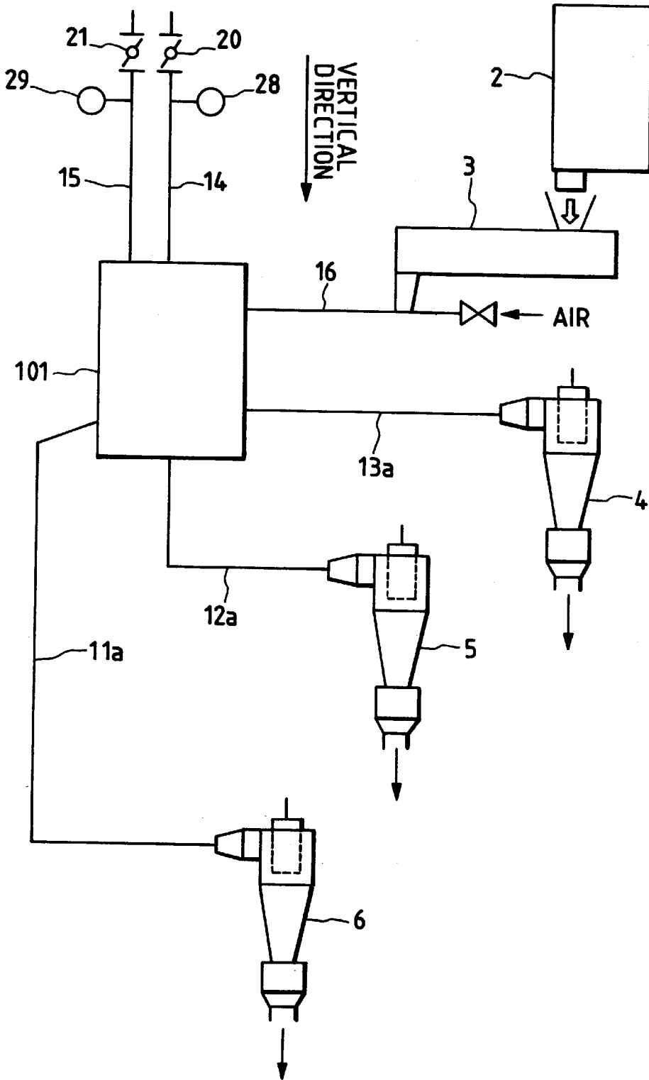
FIG. 18 PRIOR ART
