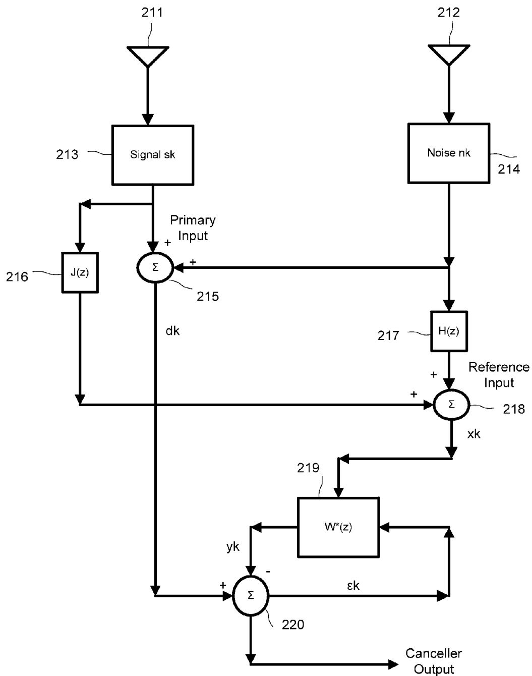
FIG. 2 PRIOR ART
