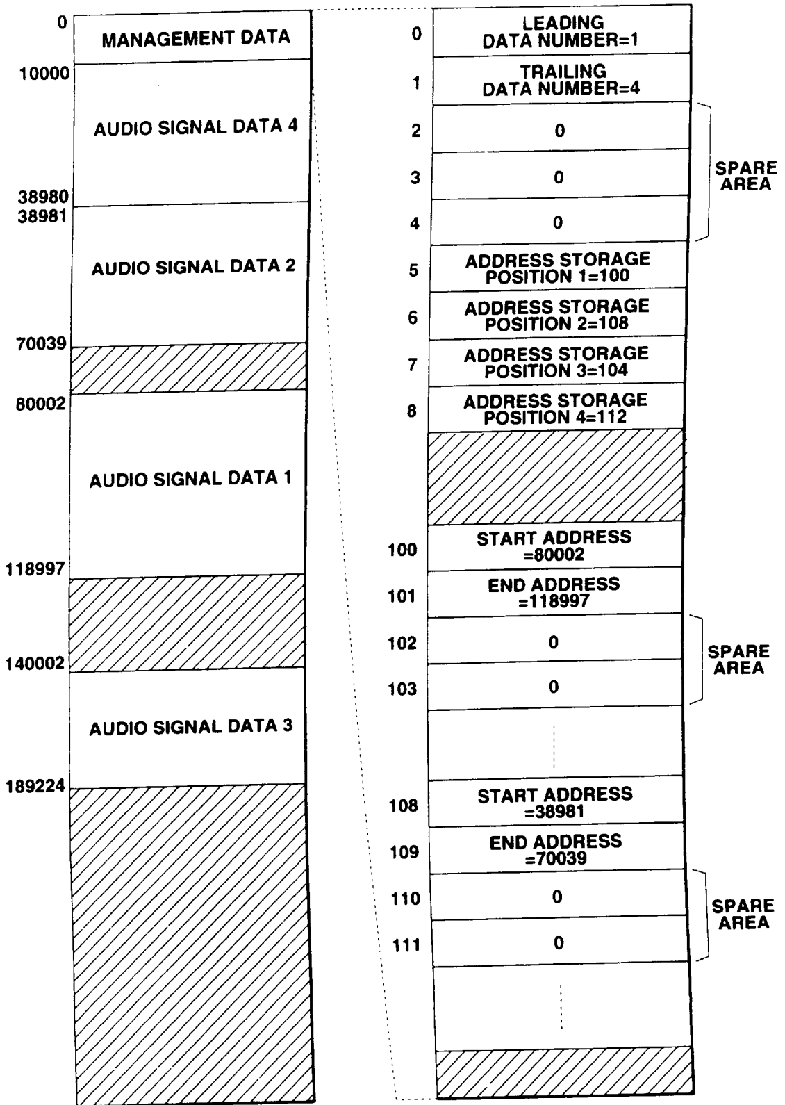
FIG.2 (PRIOR ART)
