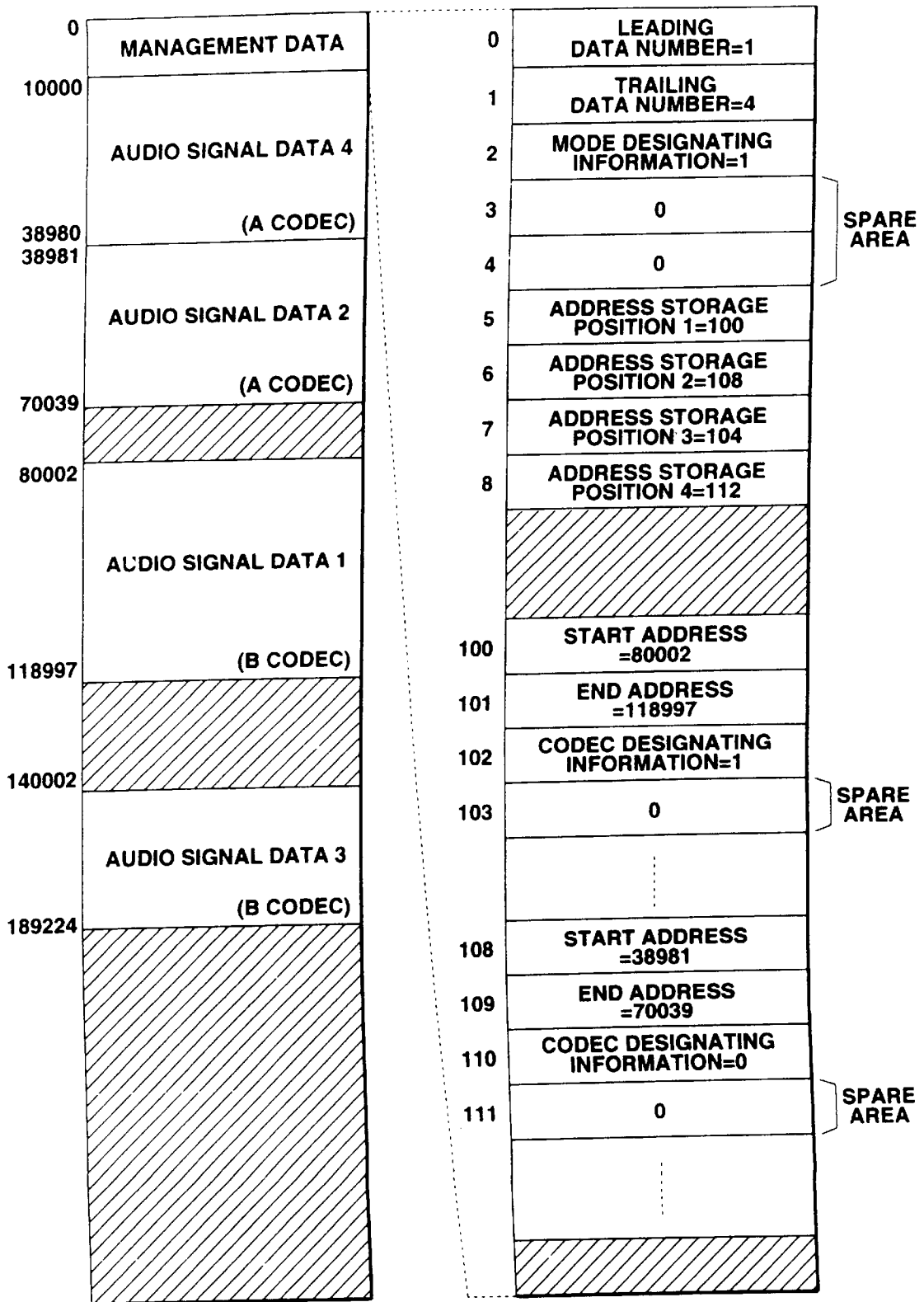
FIG.3 (PRIOR ART)
