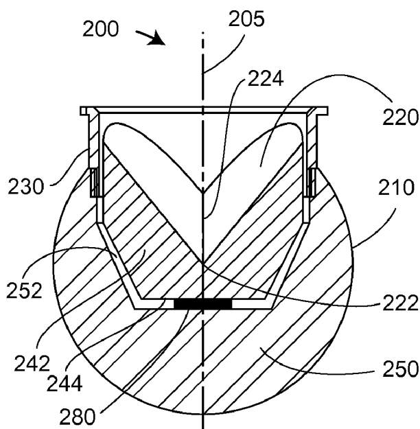
SECTION B-B FIG. 2C
