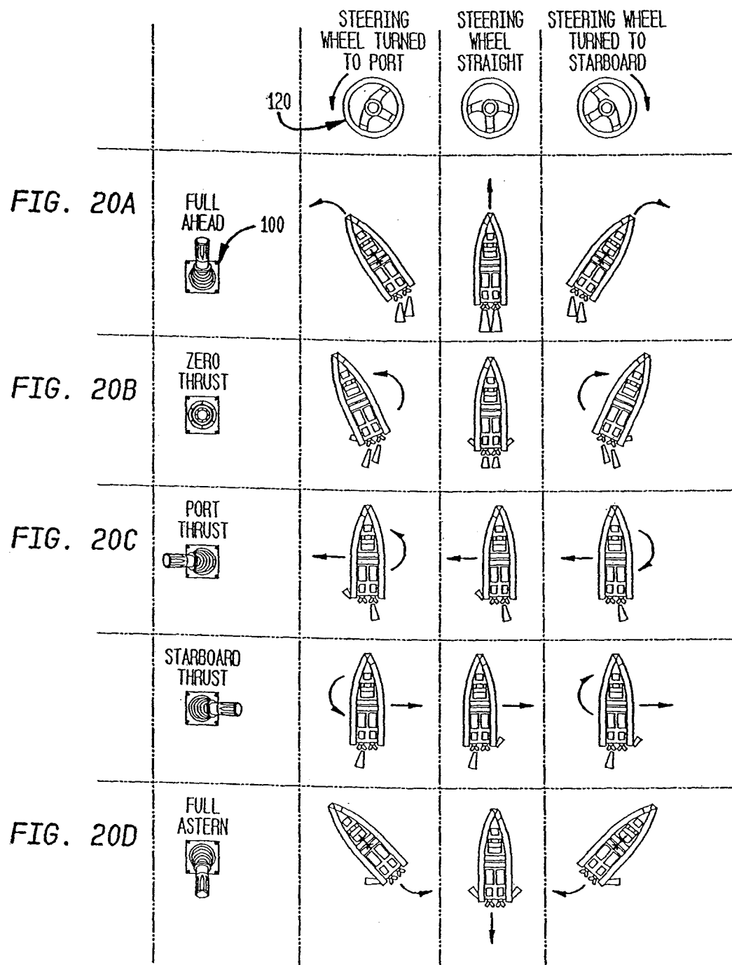
FIG. 20 DUAL WATERJET MOTION DIAGRAM
