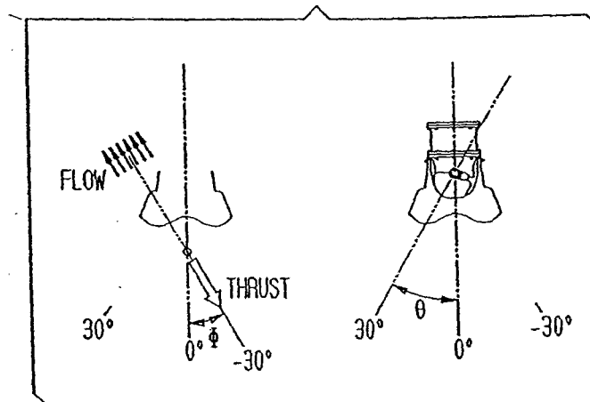
FIG. 25B FULL REVERSE BUCKET
