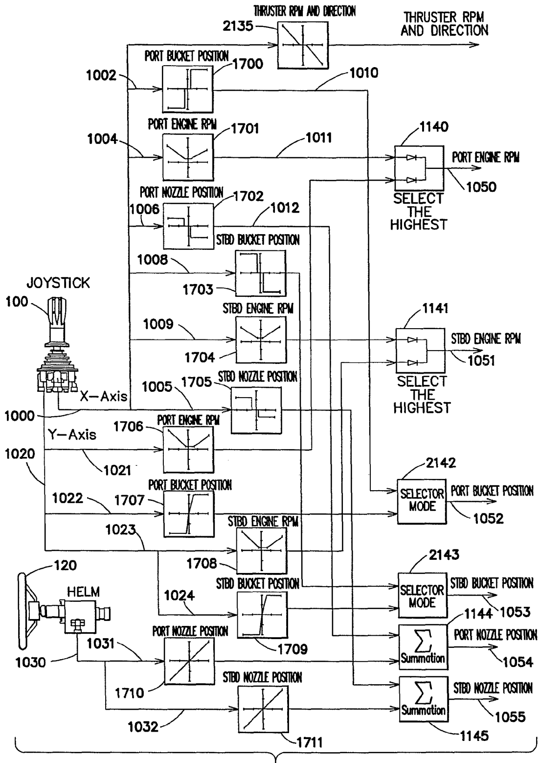
TWIN WATERJET SIGNAL DIAGRAM WITH BOWTHRUSTER
