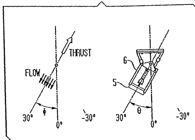
FIG. 22A FULL AHEAD BUCKET
