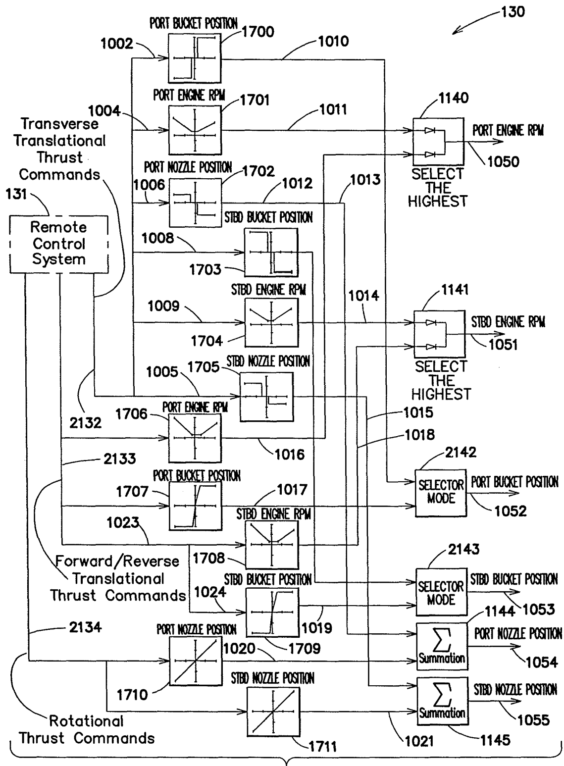
TWIN WATERJET SIGNAL DIAGRAM REMOTELY CONTROLLED
