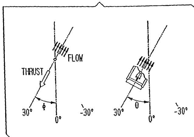
FIG. 22B FULL REVERSE BUCKET
