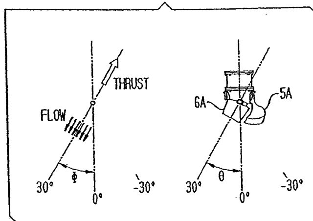
FIG. 25A FULL AHEAD BUCKET
