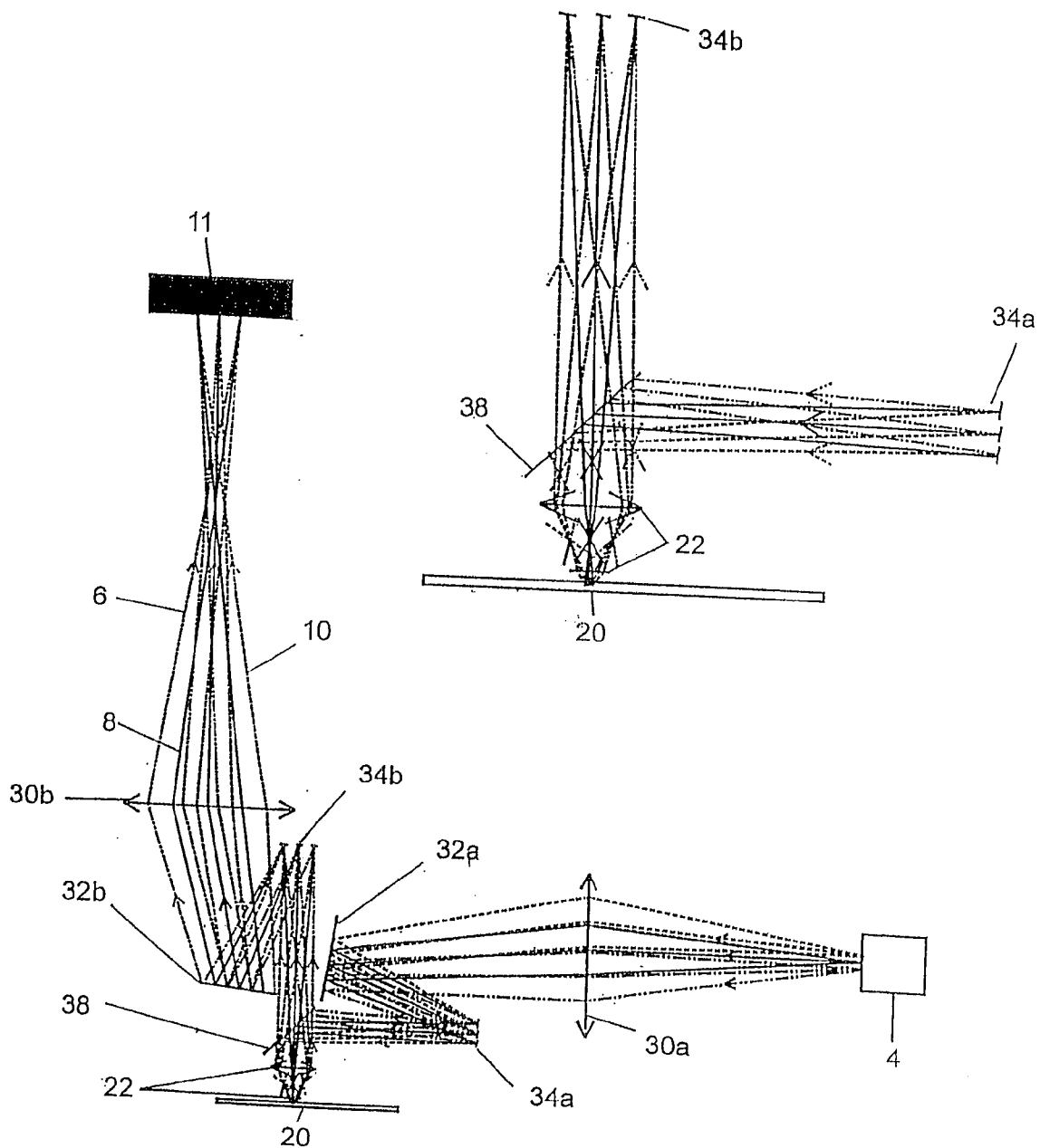
Expanded View of Digital Micromirror Devices, Dichroic Mirror, Objective Lenses and Sample
