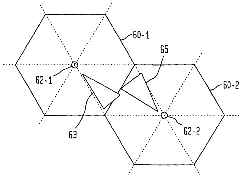
FIG. 6 (PRIOR ART)
