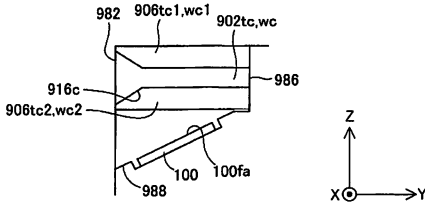
28-28 CROSS SECTION VIEW
