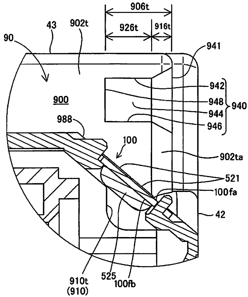
19b-19b CROSS SECTION VIEW
