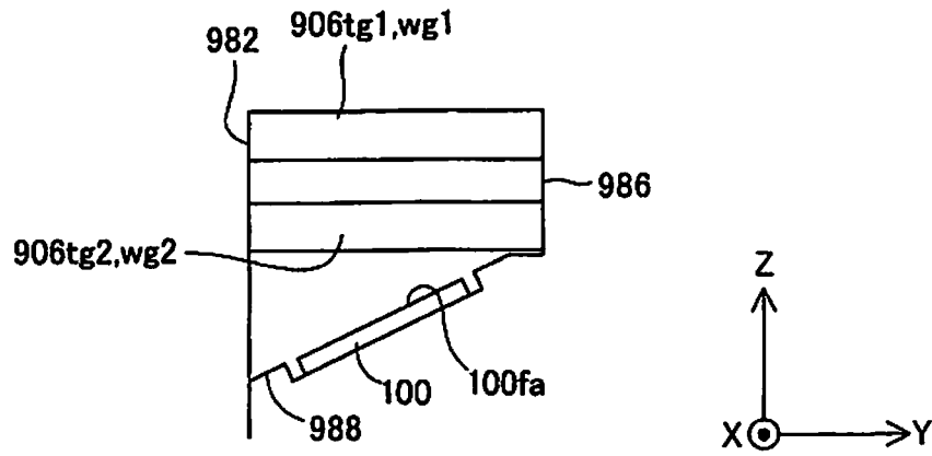
32-32 CROSS SECTION VIEW
