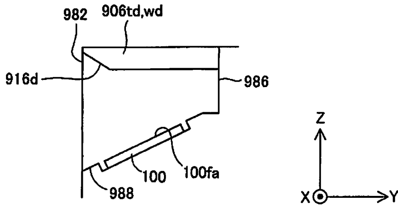
29-29 CROSS SECTION VIEW
